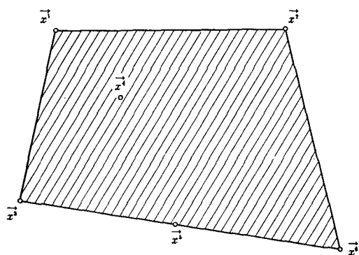
Shaded area: Convex spanned by \vec{x}^1, \dots, \vec{x}^i
